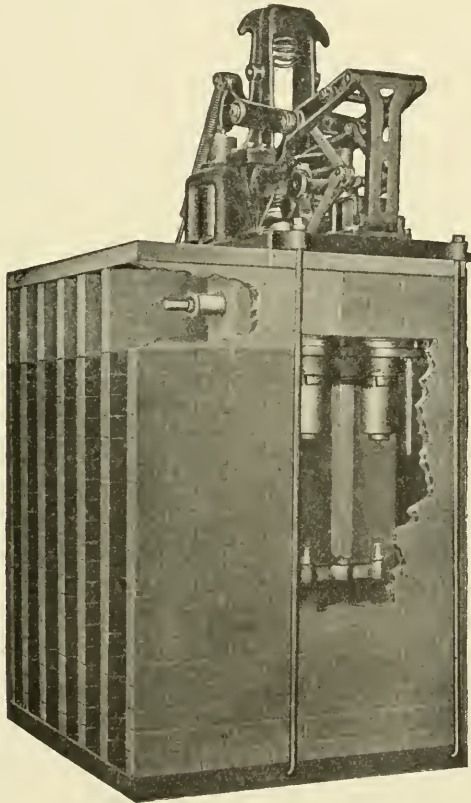
Fig. 160. Side View of Fig. 159 Showing Contact Mechanism
